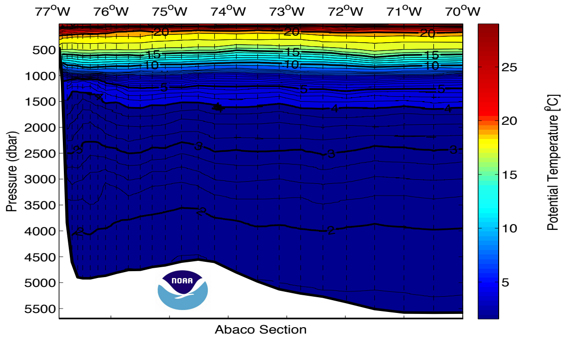
Figure 4. CTD potential temperature section off Abaco, along 26.5°N. Sept. 26 - Oct. 1, 2012.
