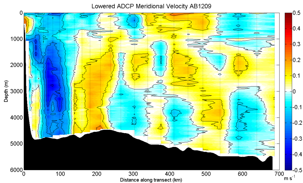
Figure 3. Absolute velocity section from LADCP off Abaco, along 26.5°N, Sept. 26 - Oct. 1, 2012.
