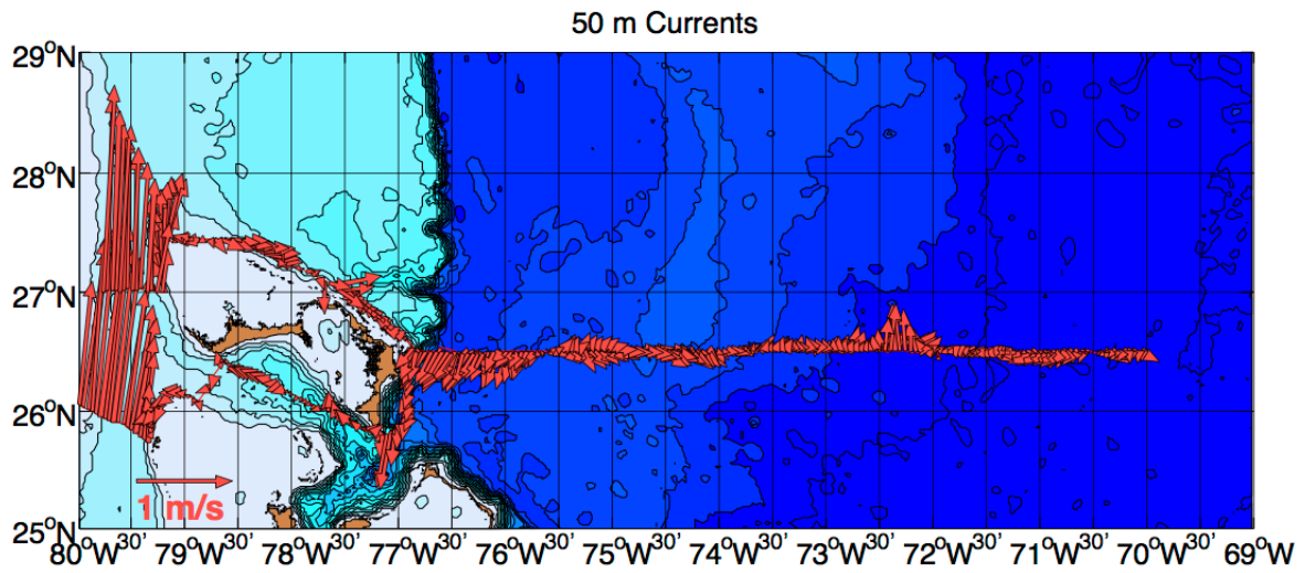
Figure 5. Currents at 50 m along the cruise track, derived from the vessel-mounted ADCP.
