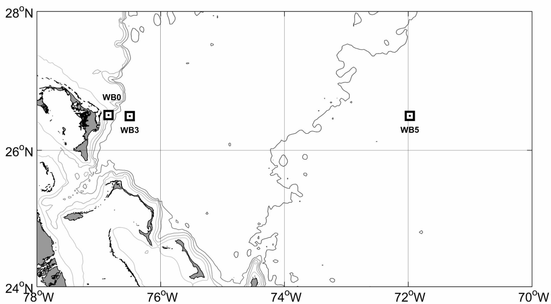
Figure 1. Current meter moorings recovered and deployed on EN-517. Additional "bottom lander" moorings (not shown on map) were deployed near mooring sites WB3, and WB5.
